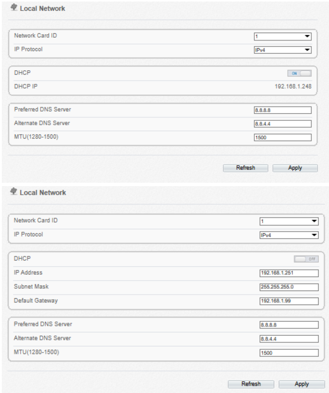
Figure 4-5 Local Network Page
