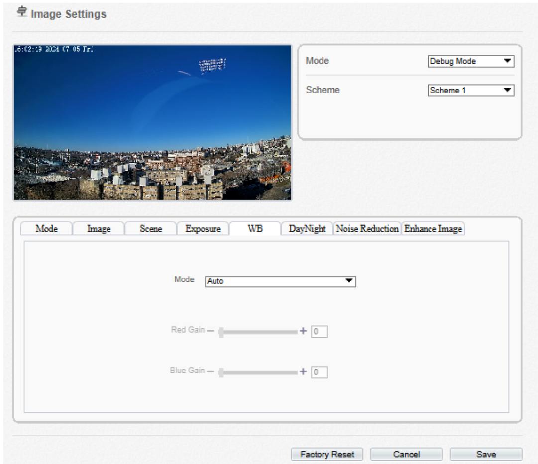
Figure 3-6 WB Setting Interface
