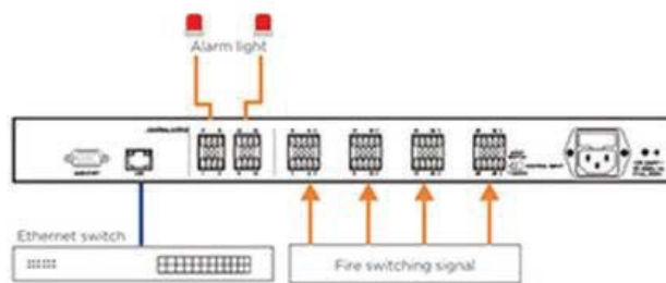
Connection Diagram
